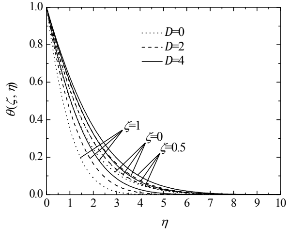
Figure(9): Effect of D and \zeta on the temperature profile ( n=0.5, I=1, R=V=0 ).
