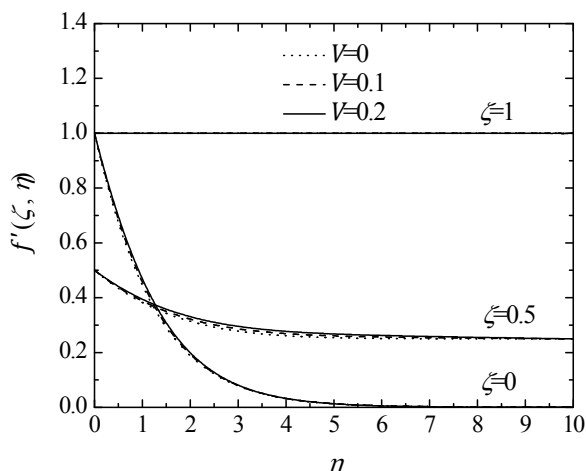
Figure(14): Effect of V and \zeta on the velocity profile ( n=0.5, I=D=R=0 ).
