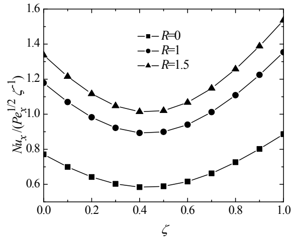
Figure(13): Effect of R and \zeta on the local Nusselt number ( n=0.5, I=D=V=0 ).
