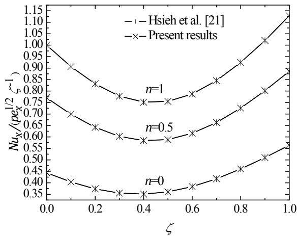
Figure(4): Effect of n and \zeta on the local Nusselt number ( I=D=R=V=0 ).
