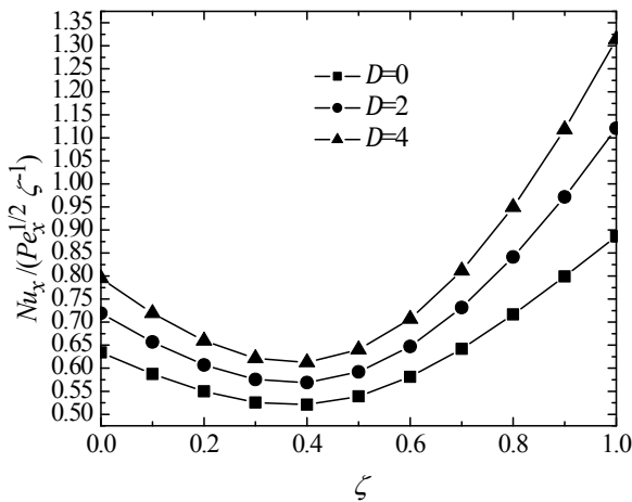
Figure(10): Effect of D and \zeta on the local Nusselt number ( n=0.5, I=1, R=V=0 ).
