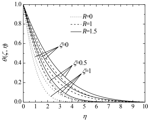
Figure(12): Effect of R and \zeta on the temperature profile ( n=0.5, I=D=V=0 ).
