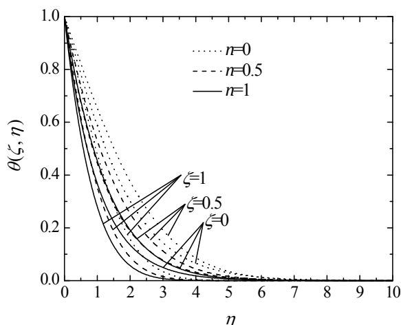
Figure(3): Effect of n and \zeta on the temperature profile ( I=D=R=V=0 ).
