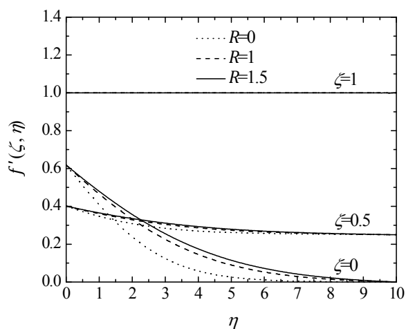
Figure(17): Effect of R and \zeta on the velocity profile ( n=0.5, I=1, D=2, V=0.1 ).
