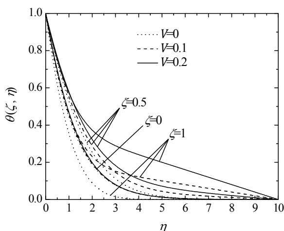
Figure(15): Effect of V and \zeta on the temperature profile ( n=0.5, I=D=R=0 ).
