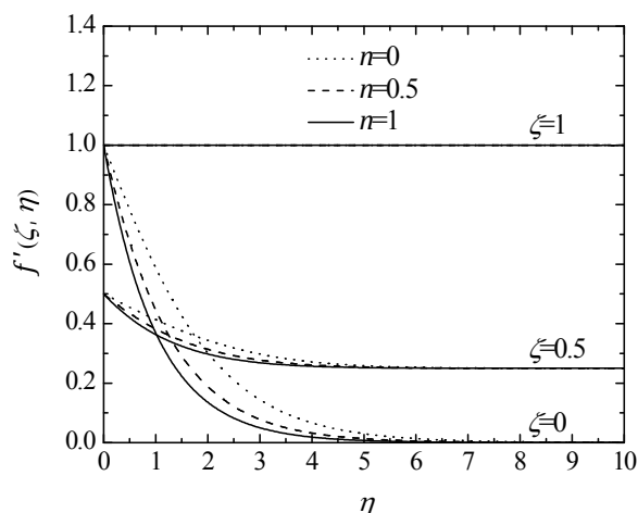
Figure(2): Effect of n and \zeta on the velocity profile ( I=D=R=V=0 ).
