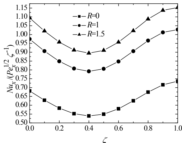
Figure(19): Effect of R and \zeta on the local Nusselt number ( n=0.5, I=1, D=2, V=0.1 ).
