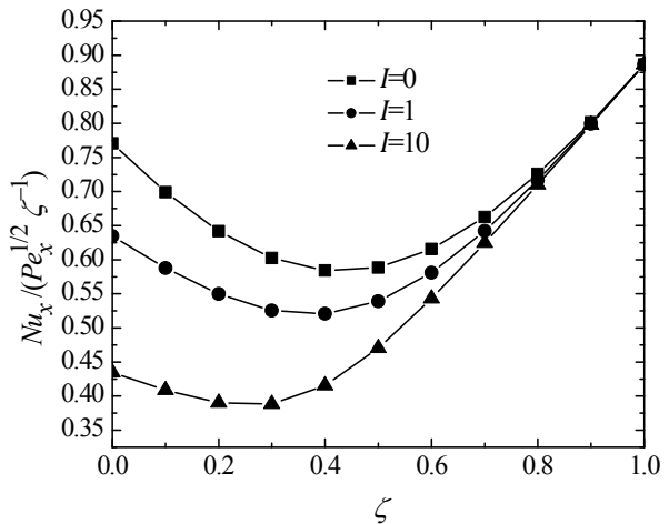
Figure(7): Effect of I and \zeta on the local Nusselt number ( n=0.5, D=R=V=0 ).
