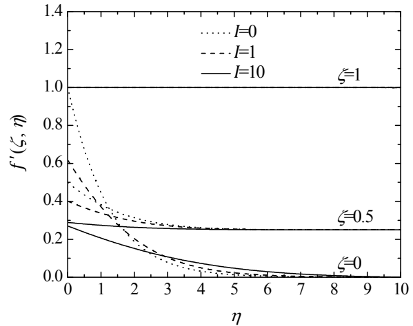
Figure(5): Effect of I and \zeta on the velocity profile ( n=0.5, D=R=V=0 ).
