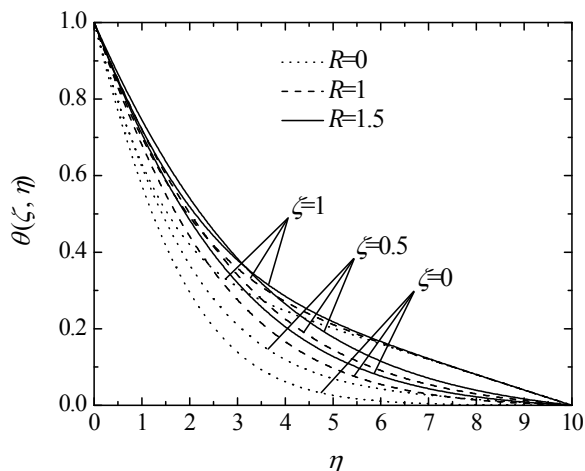
Figure(18): Effect of R and \zeta on the temperature profile ( n=0.5, I=1, D=2, V=0.1 ).
