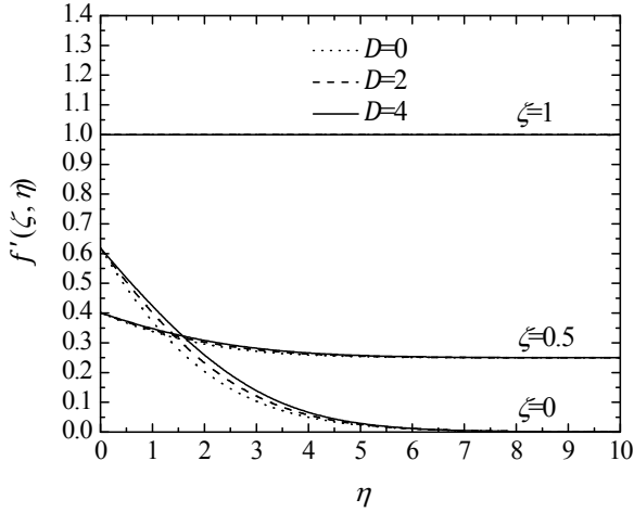
Figure(8): Effect of D and \zeta on the velocity profile ( n=0.5, I=1, R=V=0 ).
