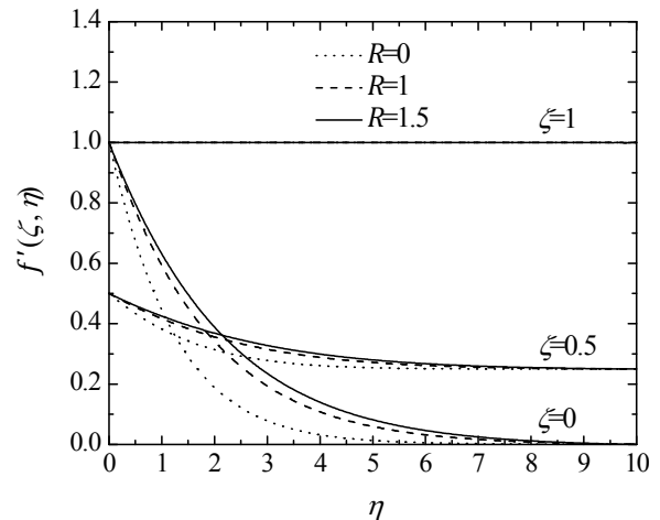
Figure(11): Effect of R and \zeta on the velocity profile ( n=0.5, I=D=V=0 ).
