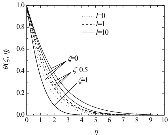
Figure(6): Effect of I and \zeta on the temperature profile ( n=0.5, D=R=V=0 ).
