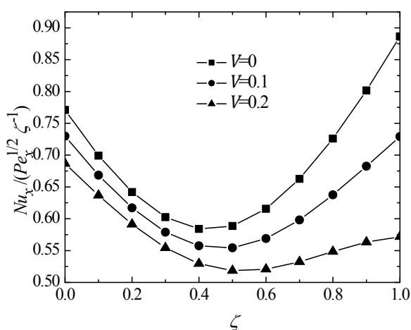
Figure(16): Effect of V and \zeta on the local Nusselt number ( n=0.5, I=D=R=0 ).
