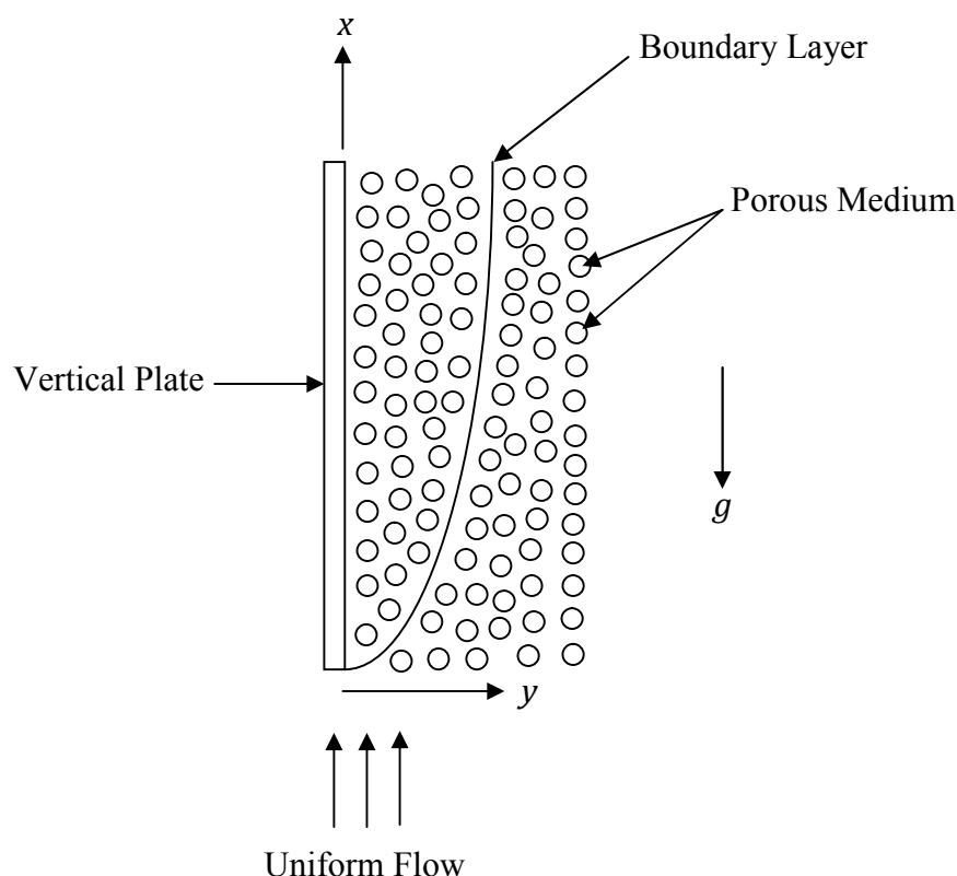
Figure(1): Physical model and coordinate system.
